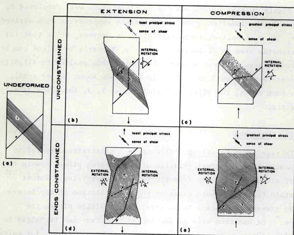
Fig. 33—Schematic illustration of internal and external rotations (from Higgs and Handin, Ref. 55, Fig. 1).
